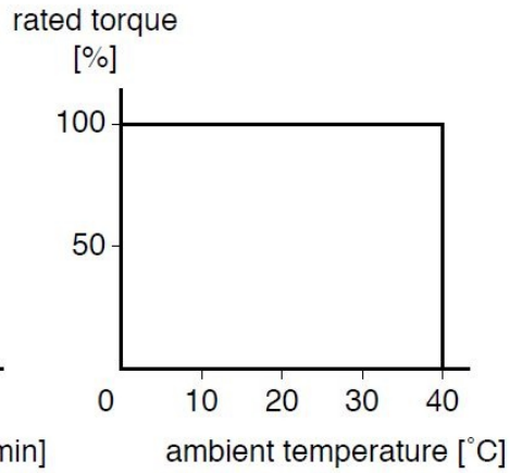
* Derating curve
