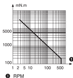
Nominal speed and torque curves 80 805 0
